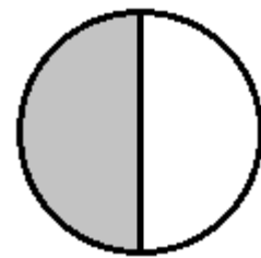
Winter Solstice
