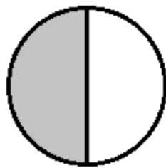
Summer Solstice
