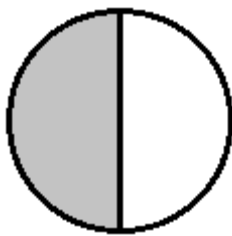
Equinoxes
